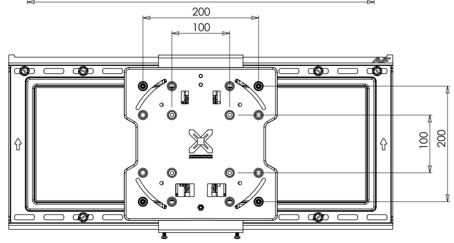
VESA CONFIGURATIONS WITHOUT ARMS
