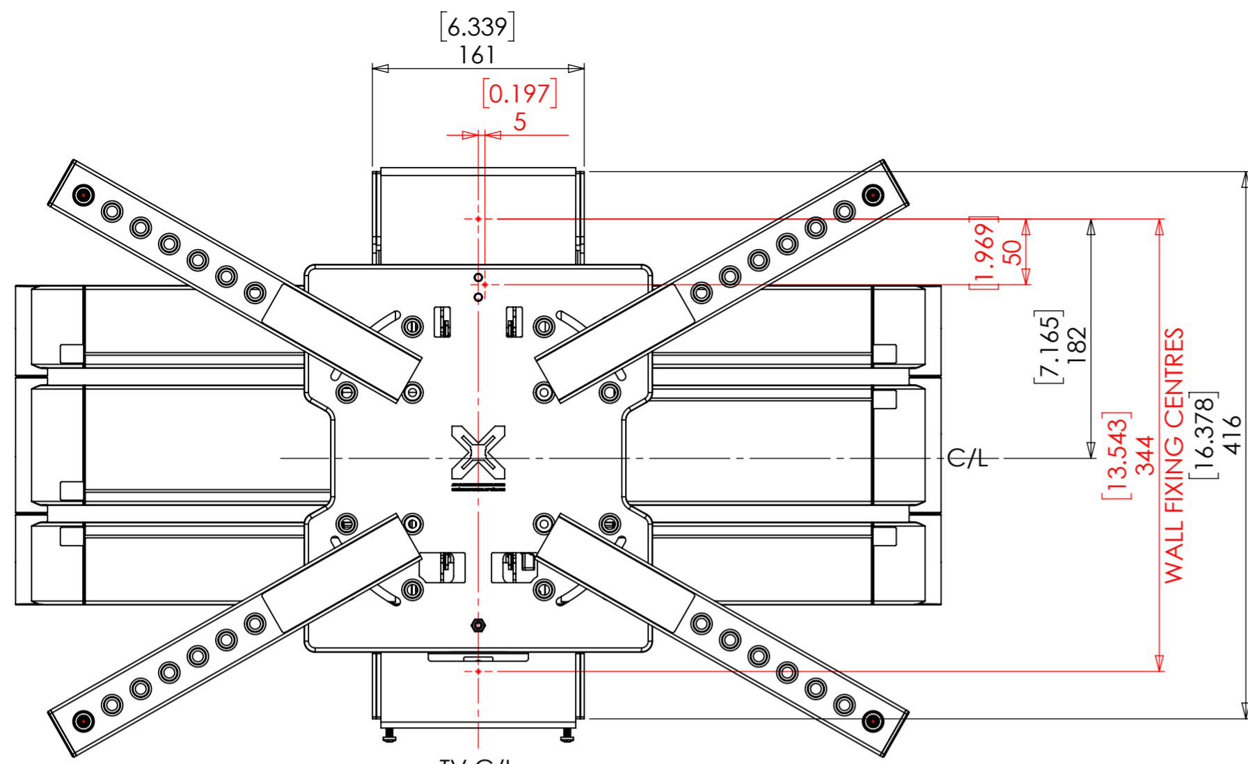
SINGLE STUD WALL FIXING OPTION
