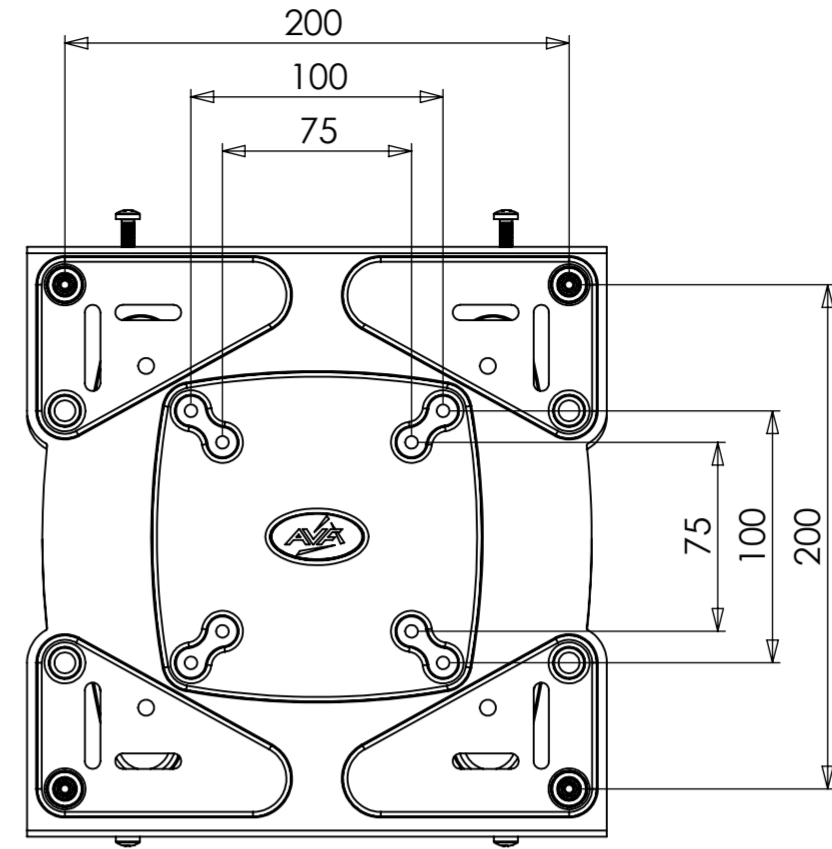
75/100/200 VESA
