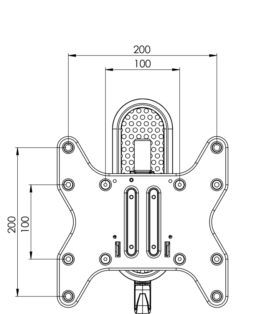
ALTERNATE FRONT PLATE
