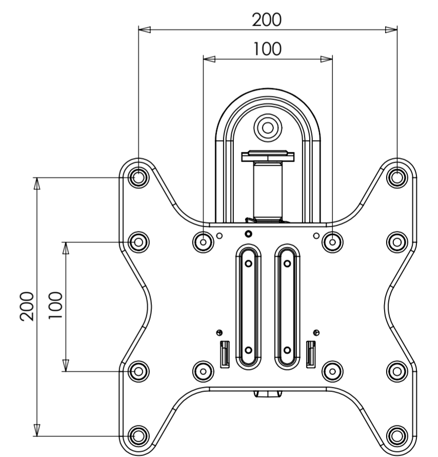
ALTERNATE FRONT PLATE
