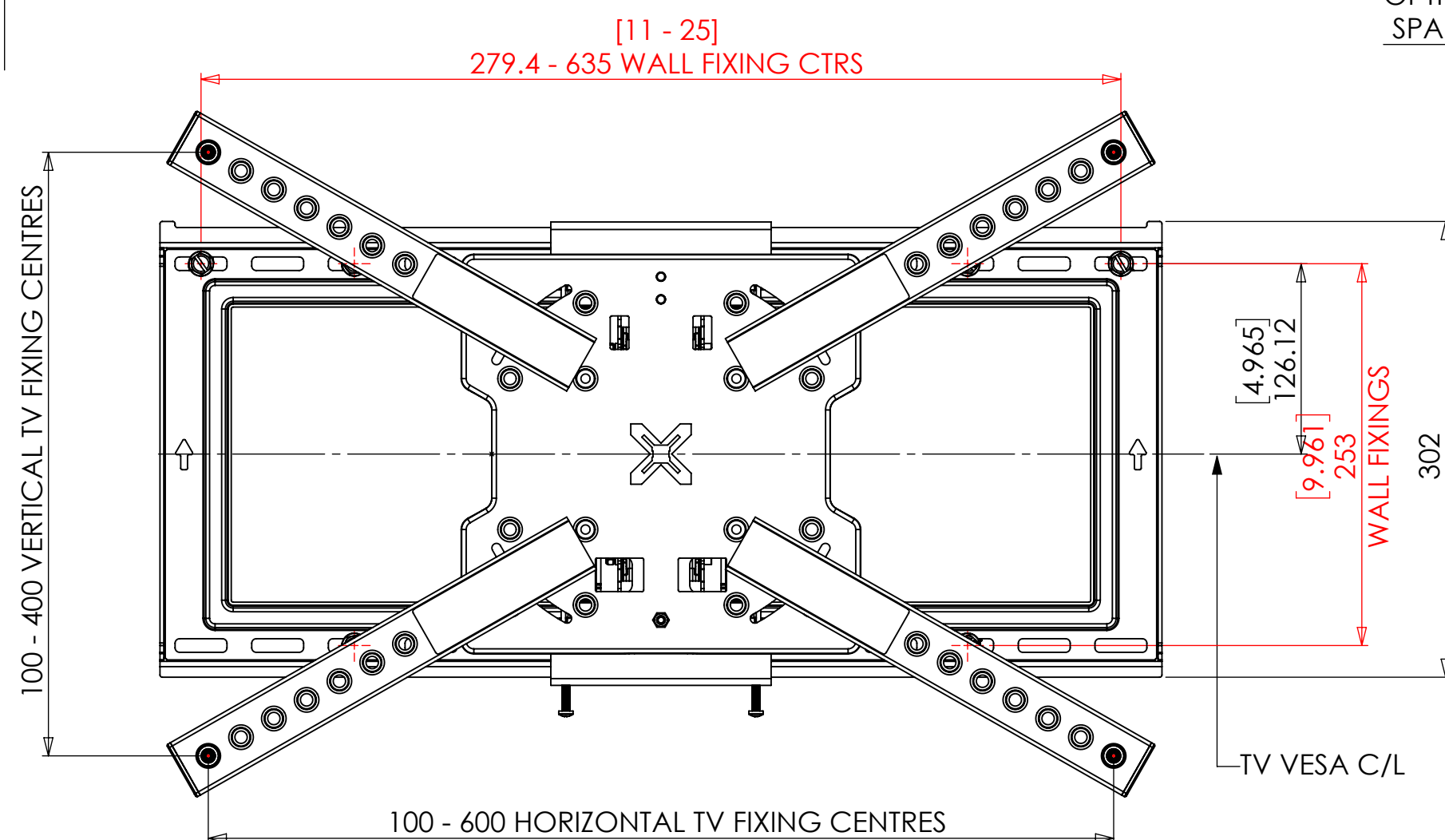
STANDARD VESA CONFIGURATION
