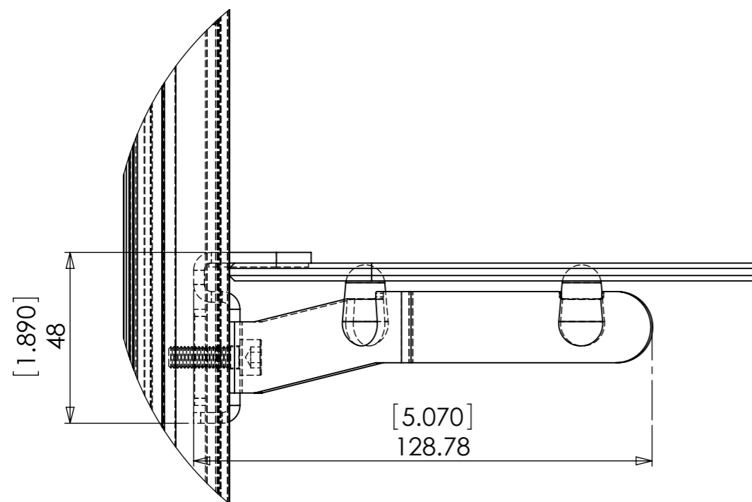
DETAIL A SCALE 2 : 3
