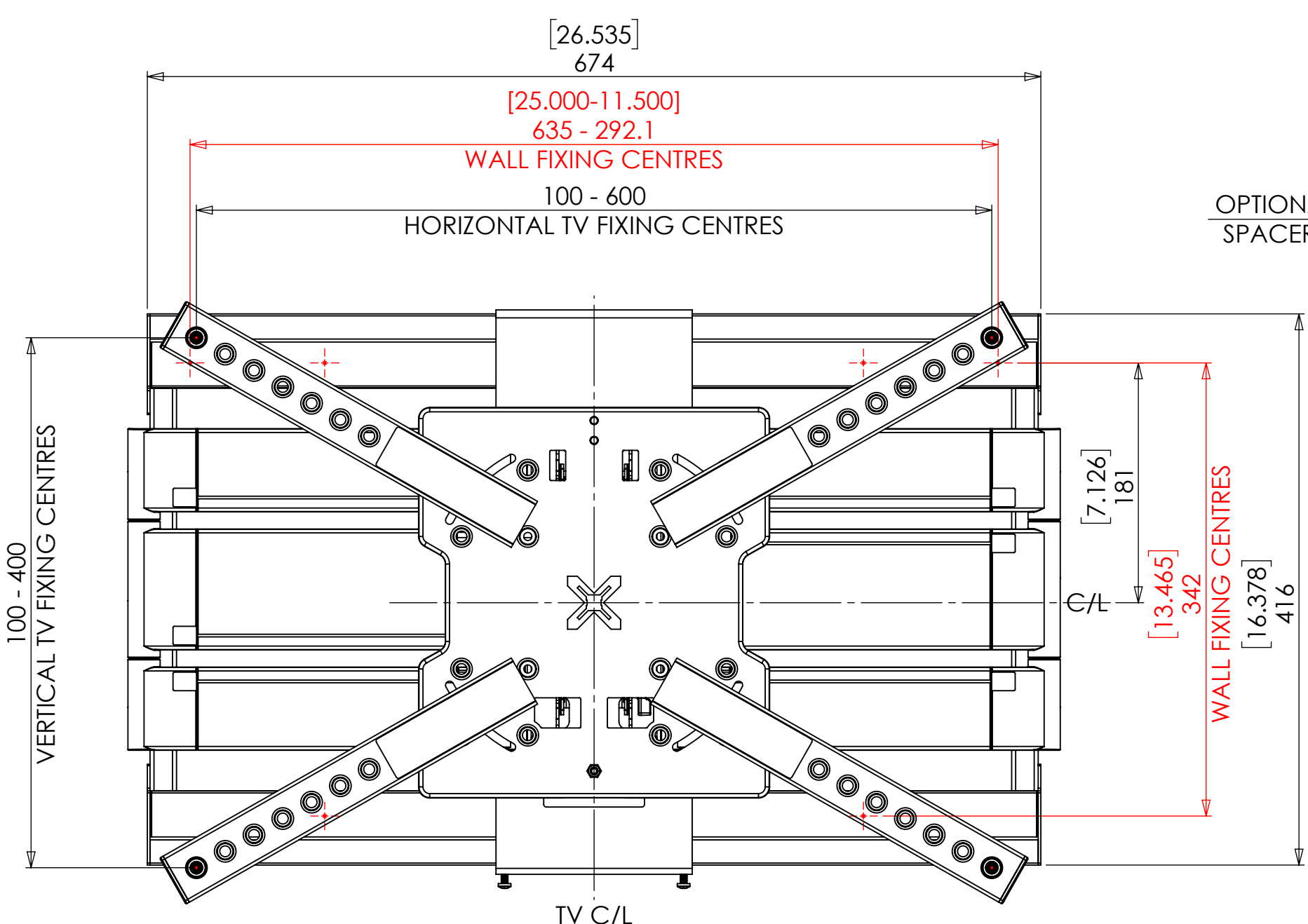
STANDARD VESA CONFIGURATION
