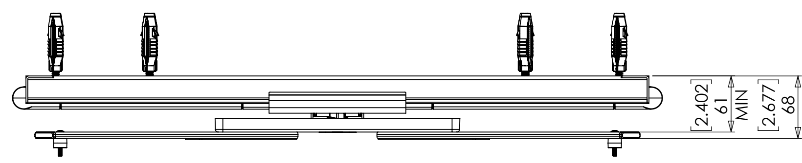
LARGE VESA CONFIGURATION
