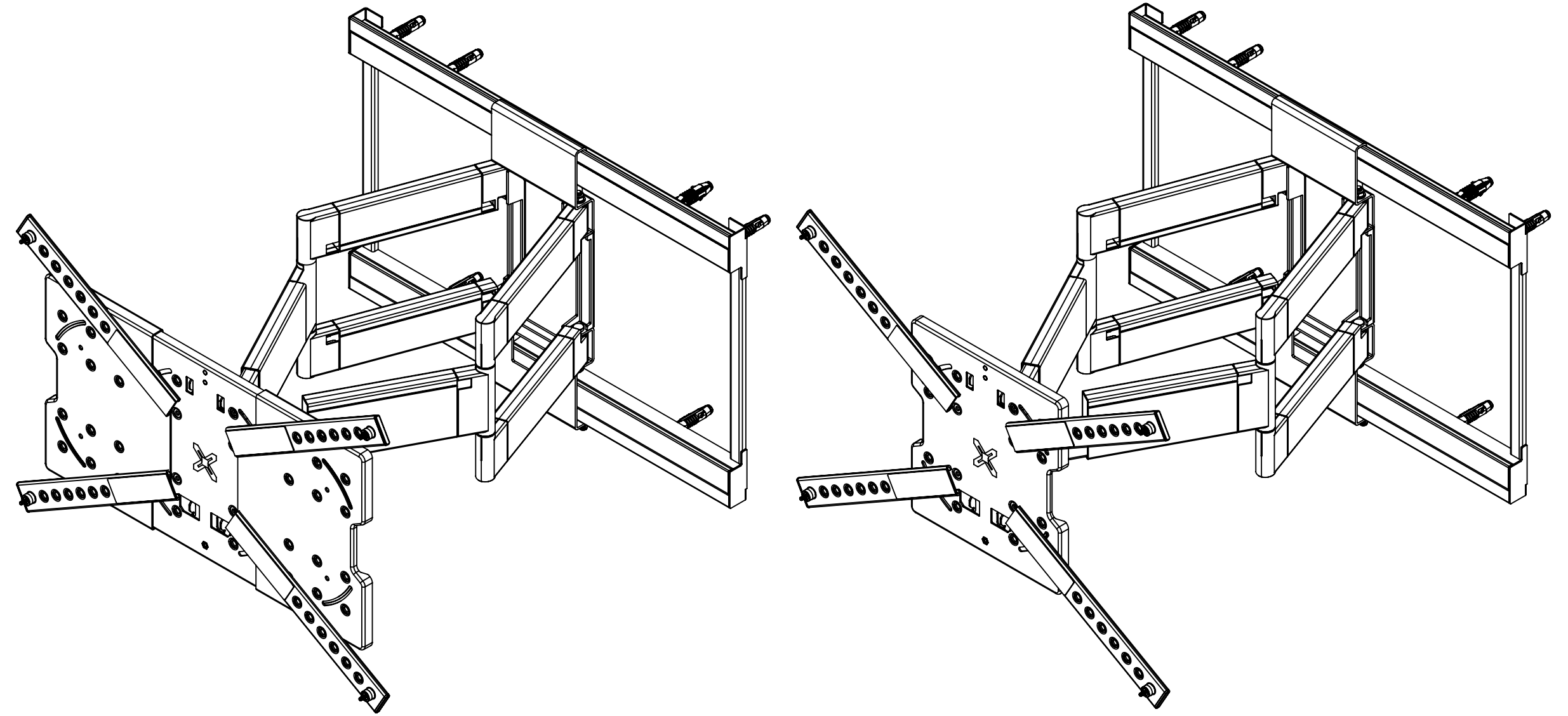
STANDARD VESA CONFIGURATION UP TO 600x400 VESA
