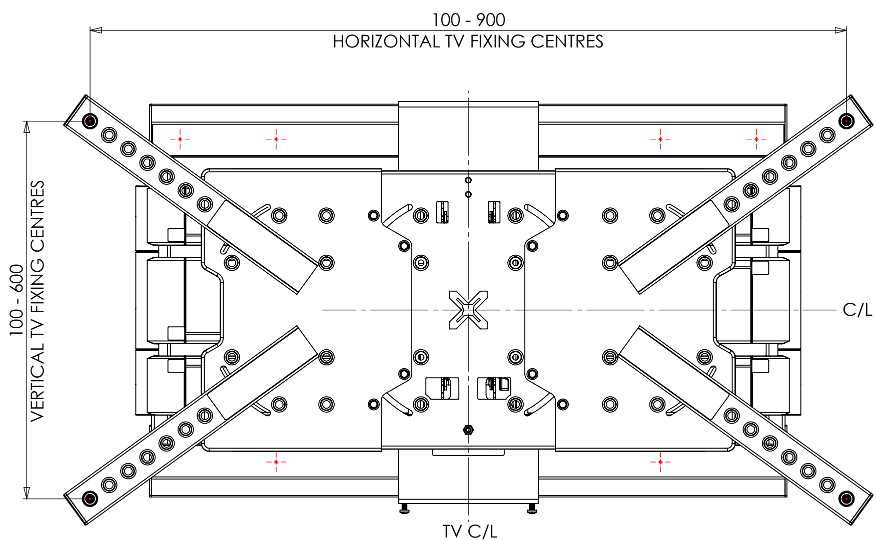
LARGE VESA CONFIGURATION
