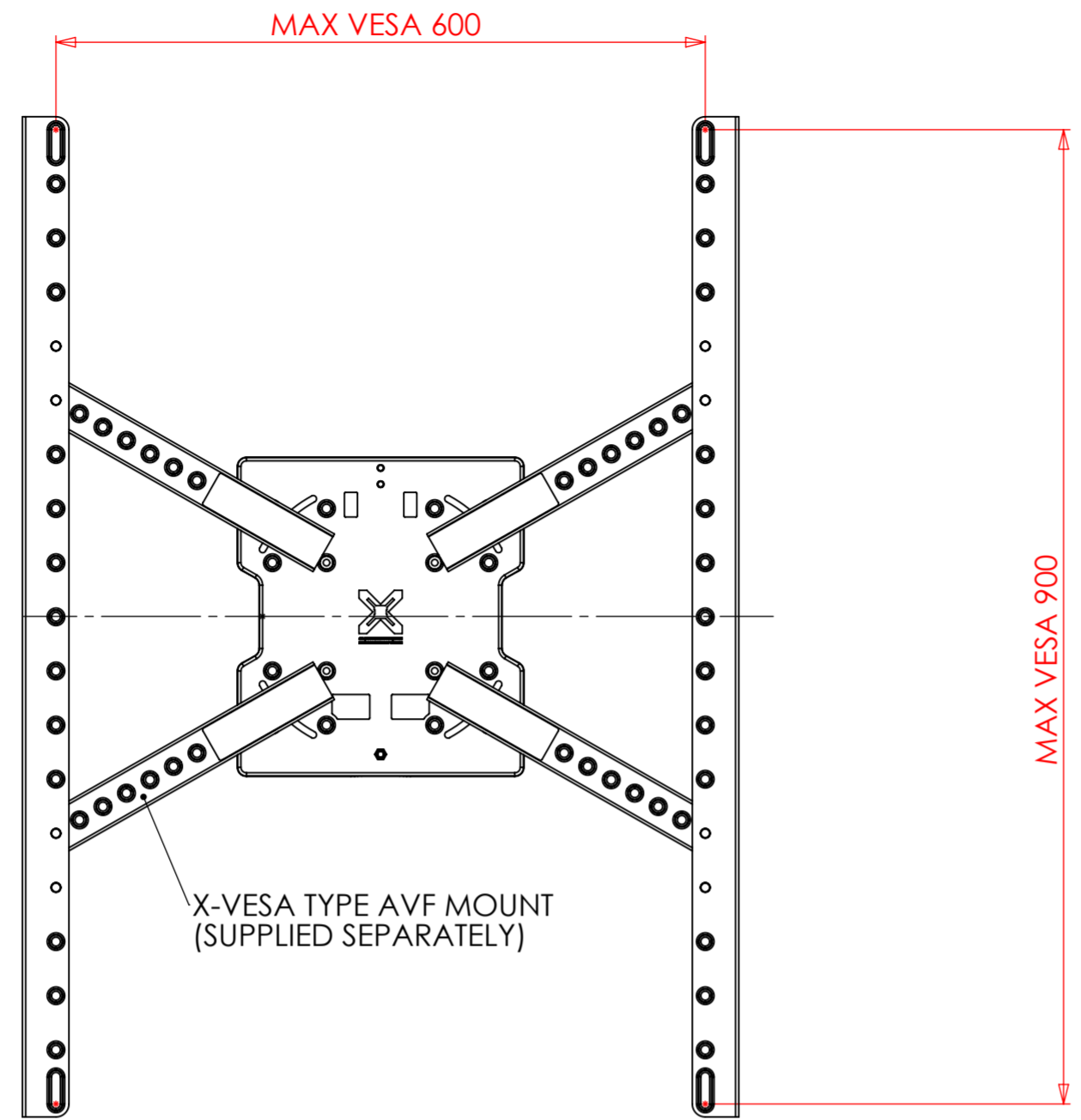
VERTICAL CONFIGURATION
