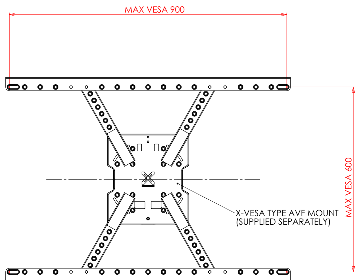
HORIZONTAL CONFIGURATION
