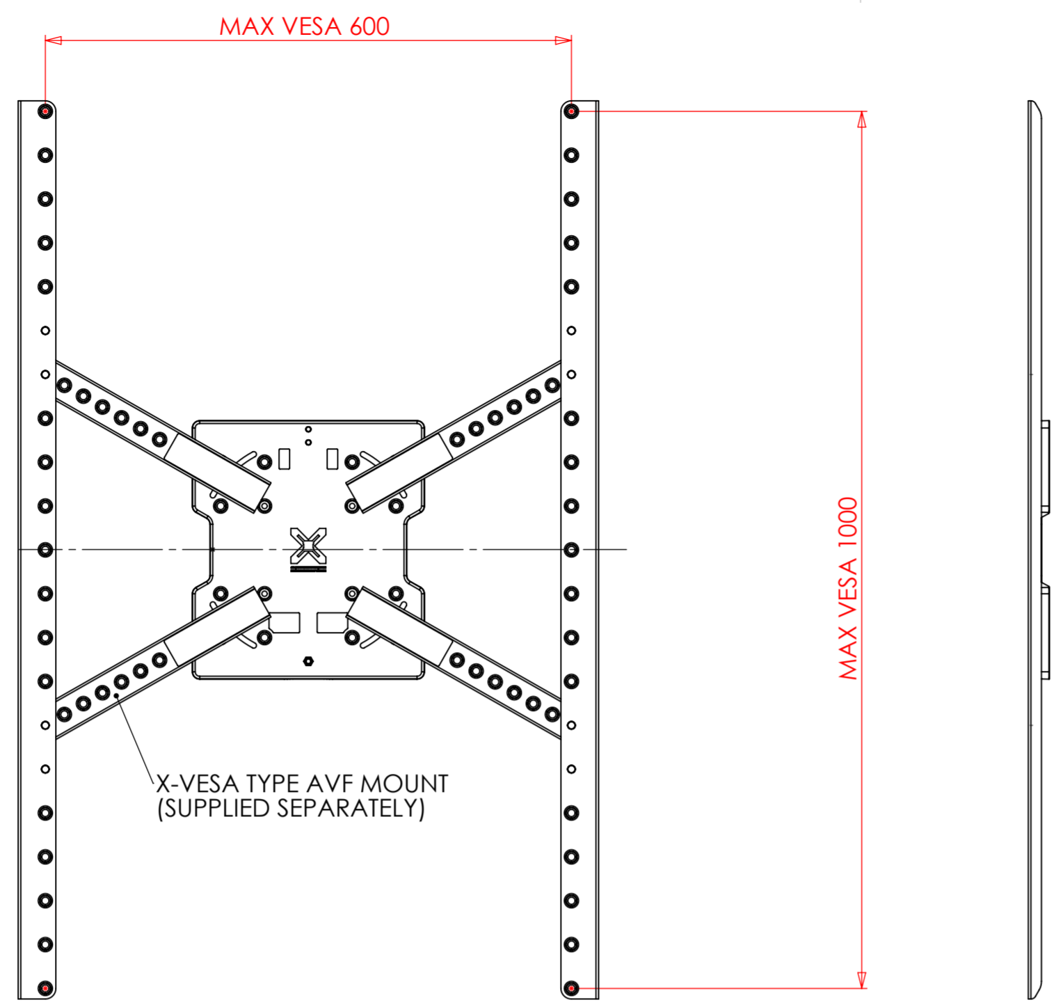
VERTICAL CONFIGURATION
