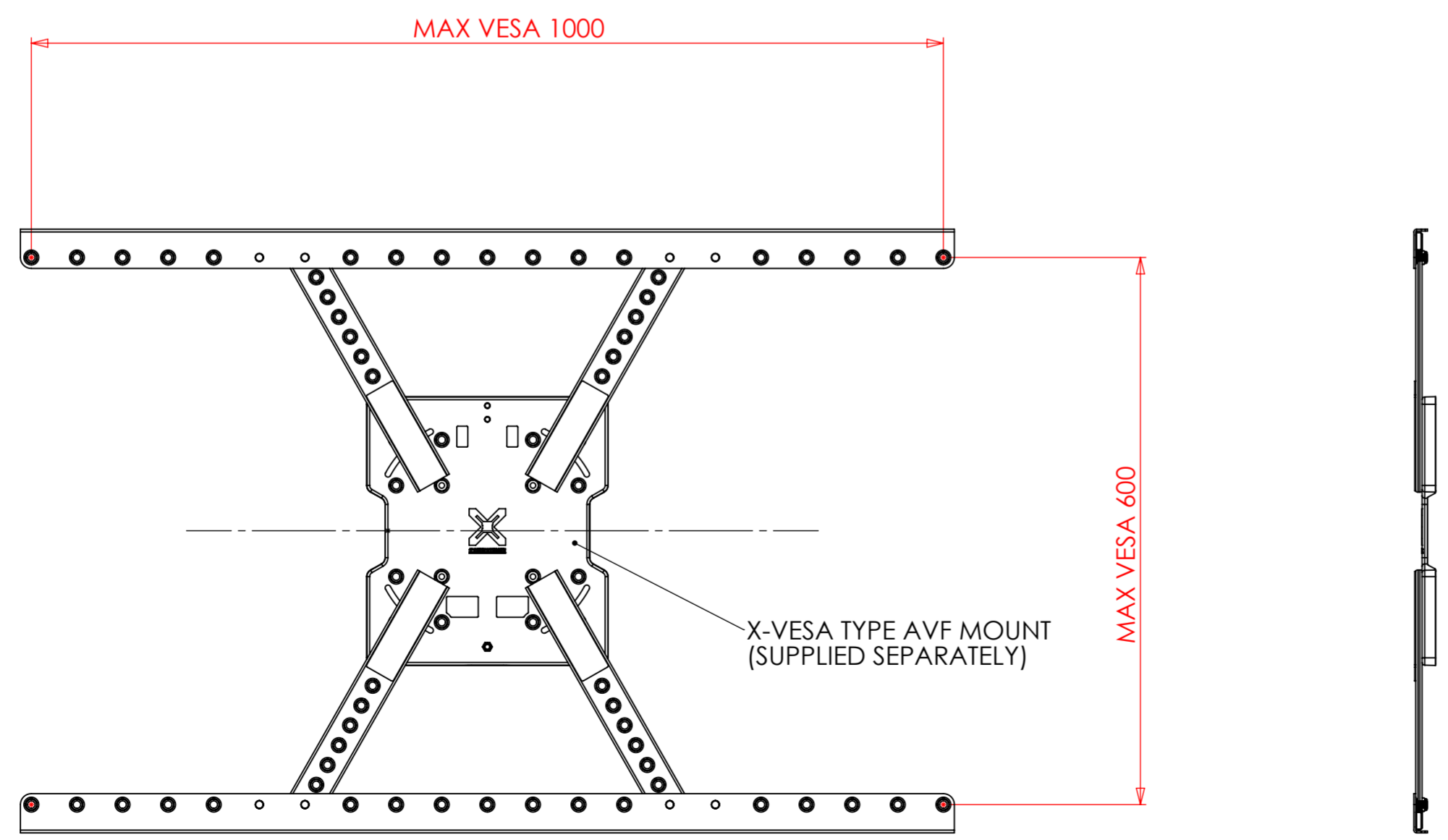
HORIZONTAL CONFIGURATION
