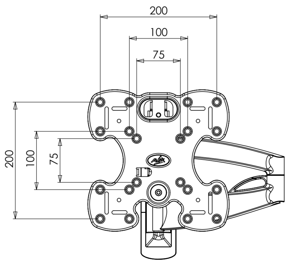
ALTERNATE VESA CONFIGURATION
