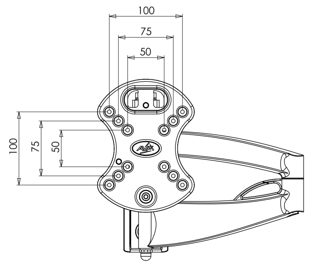
ALTERNATE VESA CONFIGURATION
