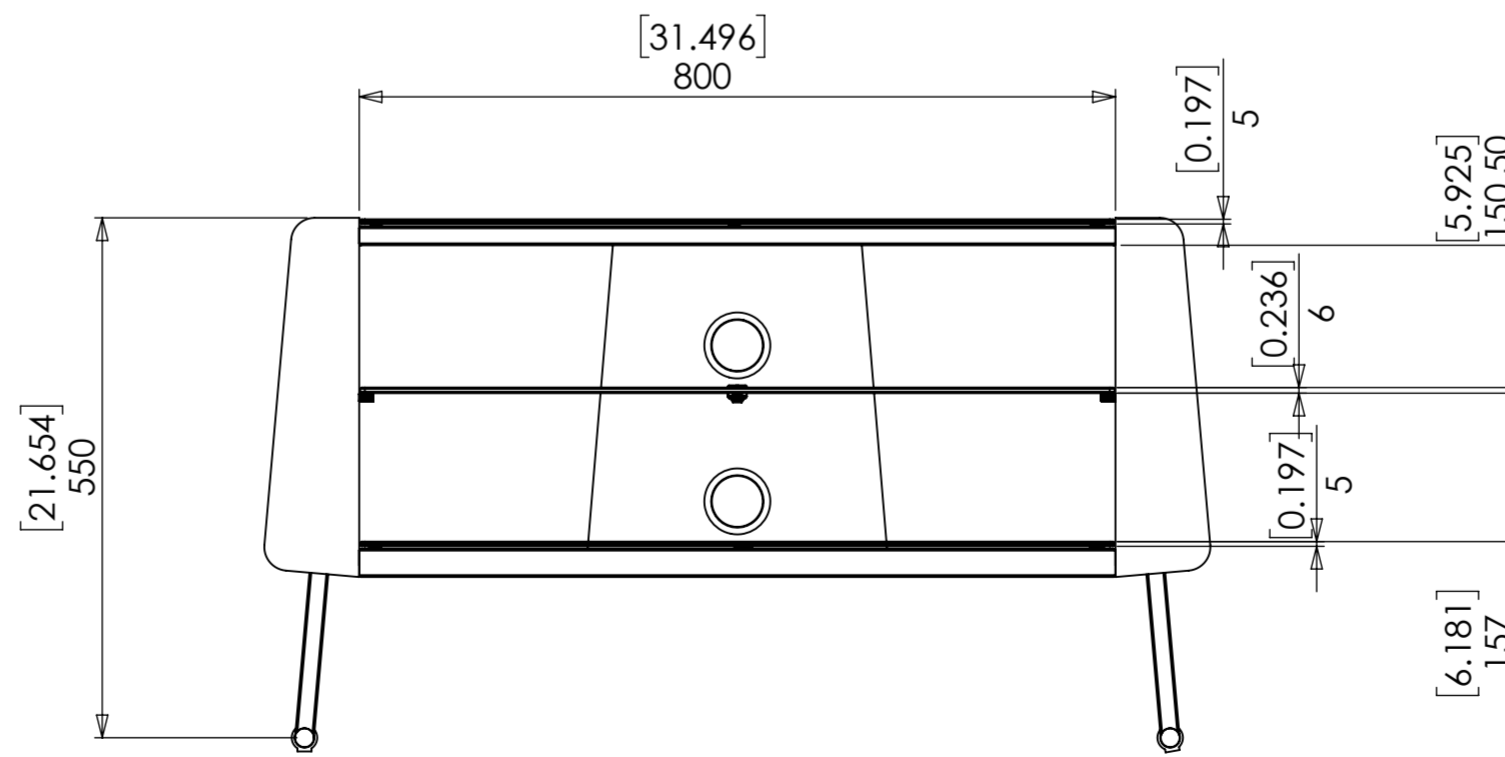
HEIGHT OPTION 3
