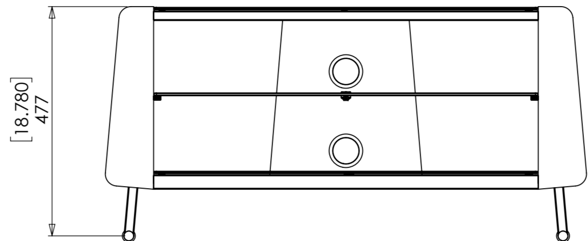
HEIGHT OPTION 2
