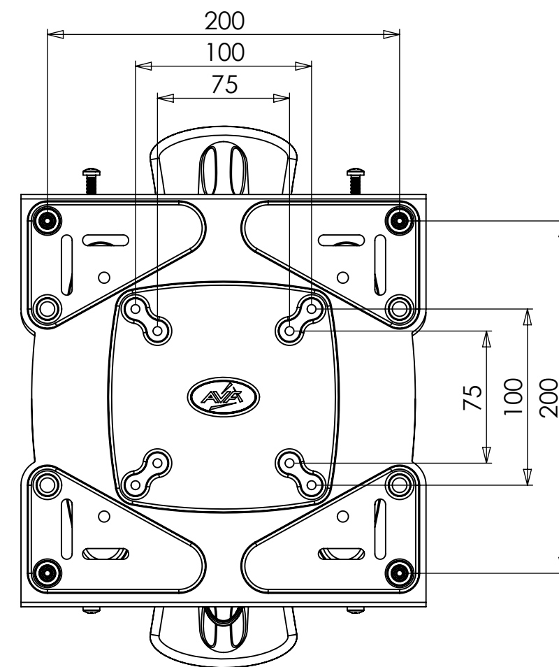
50/75/100/200 VESA
