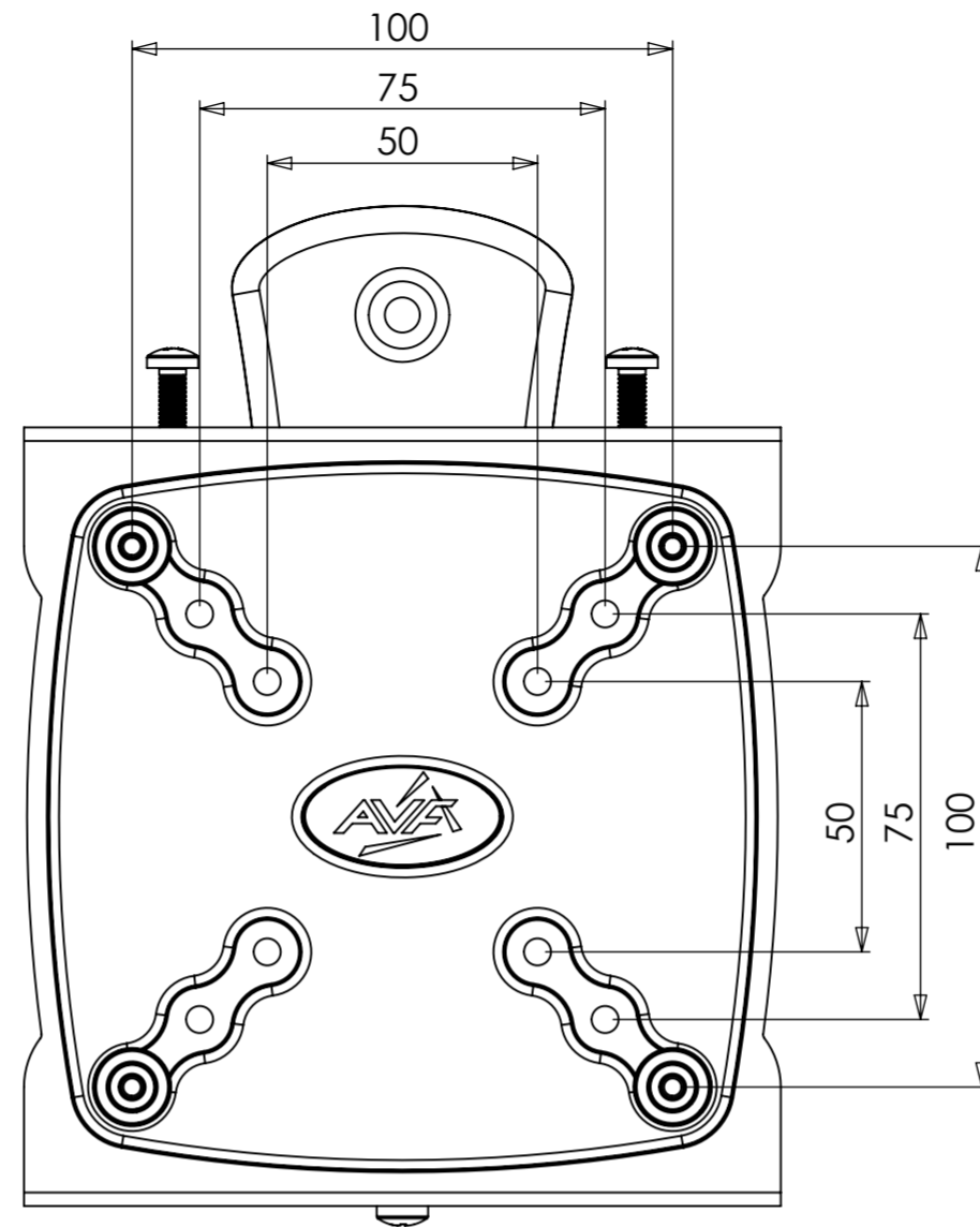
50/75/100 VESA
